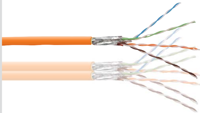
DIGITUS® Installationskabel S/FTP Cat. 7 1200 MHz, AWG 23, LSOH 1
